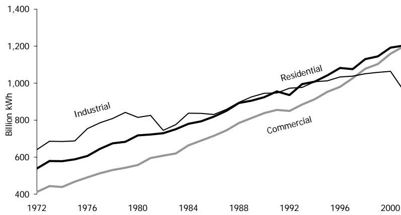
Figure 3-15: Electric Generation Retail Sales by End-Use Sector Note: The transportation end-use sector consumes minor quantities of electricity.
