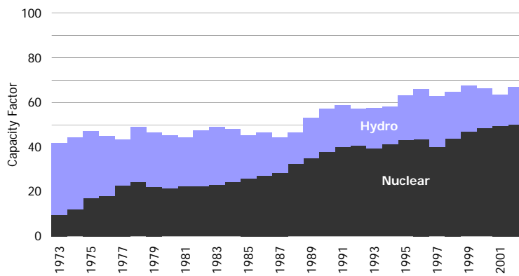
Figure 3-8: Aggregate Nuclear and Hydroelectric Power Plant Capacity Factors in the United States (1973-2002)
