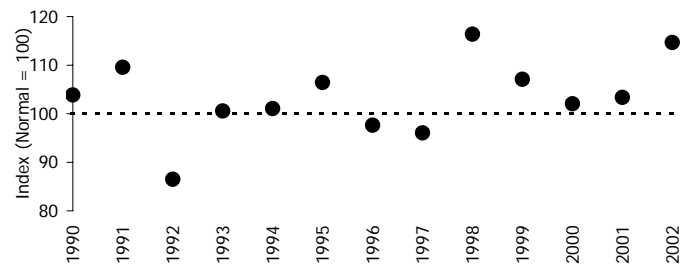
Figure 3-14: Cooling Degree Days Note: Excludes Alaska and Hawaii
