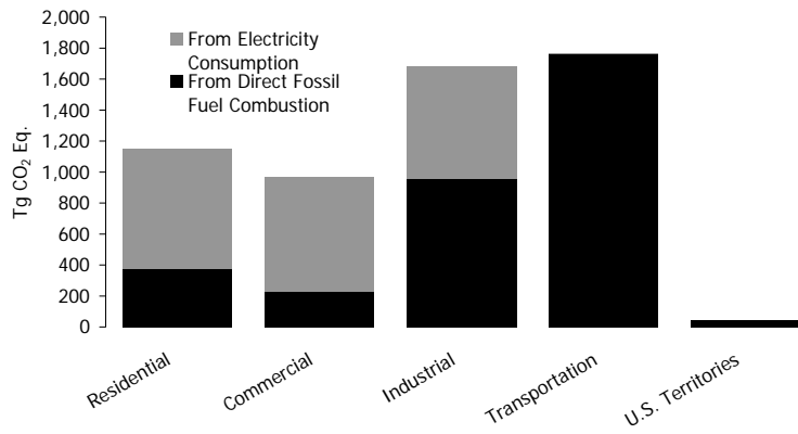
Figure 3-9: 2002 End-Use Sector Emissions of CO 2 from Fossil Fuel Combustion
