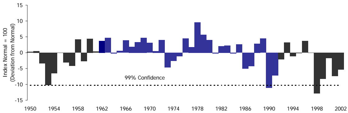
Figure 3-6. Annual Deviations from Normal Heating Degree Days for the United States (1949-2002) Note: Climatological normal data are highlighted. Statistical confidence interval for "normal" climatology period of 1961 through 1990.
