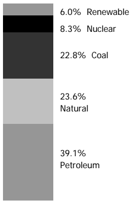
Figure 3-3: 2002 U.S. Energy Consumption by Energy Source
